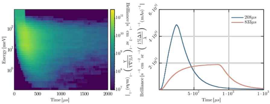
Figure V.58: Left: Energy and time dependence of the neutron brilliance at a cold extraction channel (para H 2 , length 10 cm, radius 1 cm) in forward direction for a proton pulse length of 208 μs. Right: Time structure of the neutron pulses at a 96 Hz (blue) and a 24 Hz target station (orange), respectively. The brilliance is averaged over the energy range E = 1 - 100 meV and multiplied with the repetition rate of the beam.
