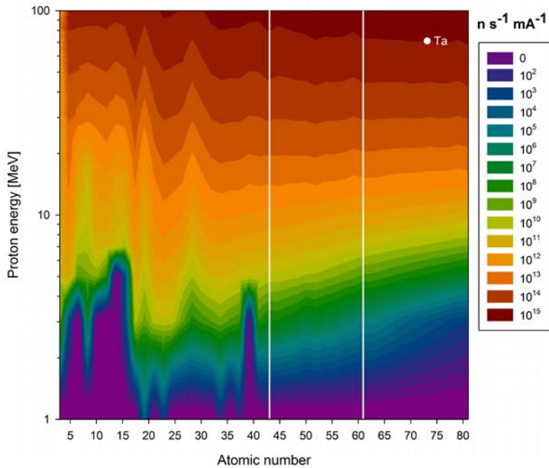
Figure V.2: Dependence of the neutron yield for protons on the atomic number Z and the primary ion energy. White lines: Tc and Pm, white dot: Ta at 70 MeV
