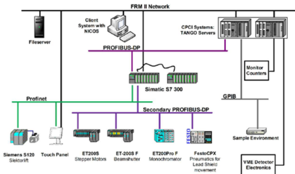
Figure VII.5: Physical architecture of the instrument control system of DNS
